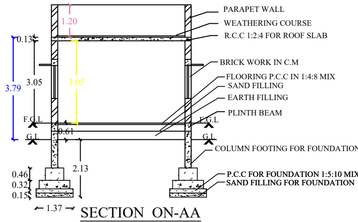
SECTION ON-AA
