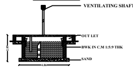
SECTION OF THE SEPTIC TANK
