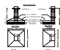
COLUMN FOOTING DETAILS
