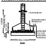
TYP.DET. COLUMN FOOTING
