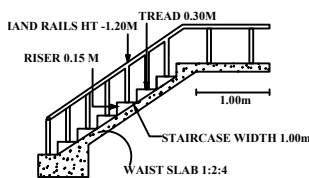
STAIRCASE DETAILS
