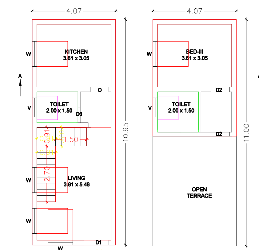
GROUND FLOOR PLAN Scale-1:100 FIRST FLOOR PLAN Scale-1:100
