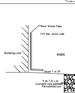
PERCOLATION PIT :
