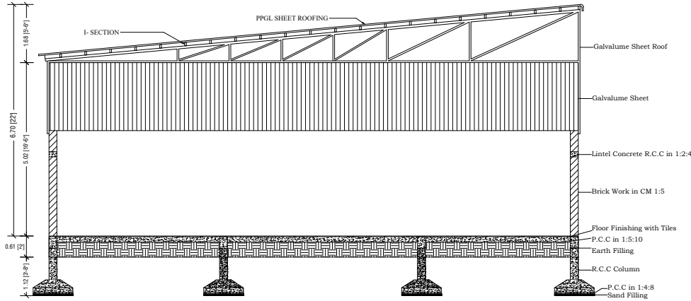
SECTION X-X
