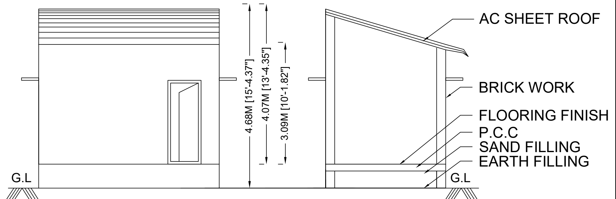
FRONT ELEVATION
