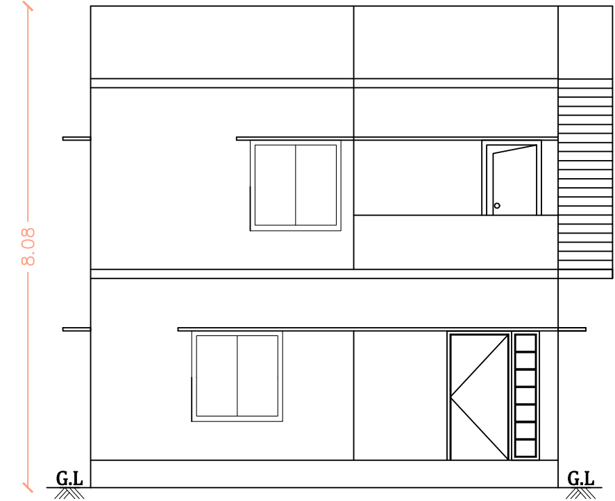
FRONT ELEVATION
