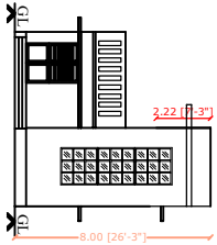
BLOCK 1 FRONT ELEVATION
