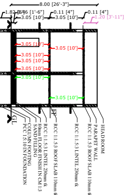
BLOCK 2 SECTION ON A-A
