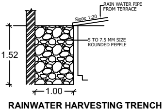
RAINWATER HARVESTING TRENCH
