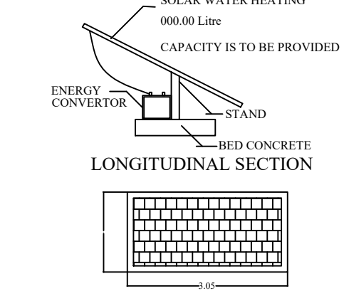
SOLAR PANEL
