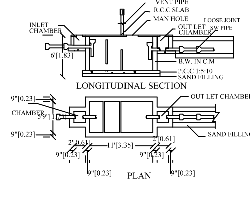
SEPTIC TANK:
