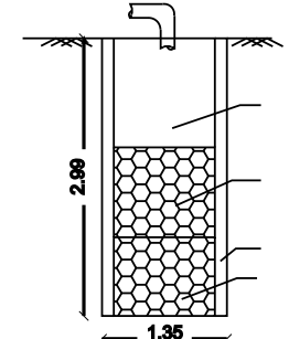
RAIN WATER COLLECTION TANK COLLECTION OF RAIN WATER FROM BUILDING
