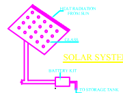
SOLAR SYSTEM
