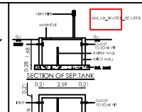
SECTION OF SEPTIC TANK
