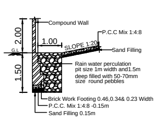
RAINWATER HARVESTING TRENCH
