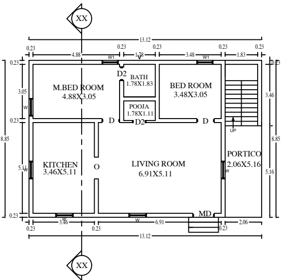
PROPOSED BUILDING OF GROUND FLOOR
