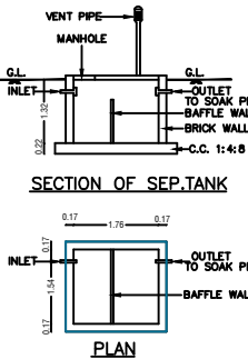
SEPTIC TANK
