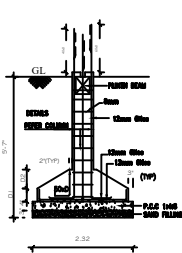
FOUNDATION DETAILS
