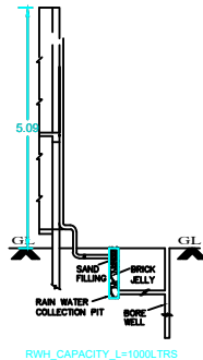
RAIN WATER HARVESTING SYSTEM
