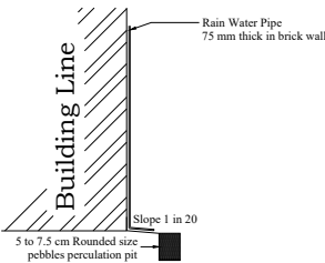
RAINWATER HARVESTING
