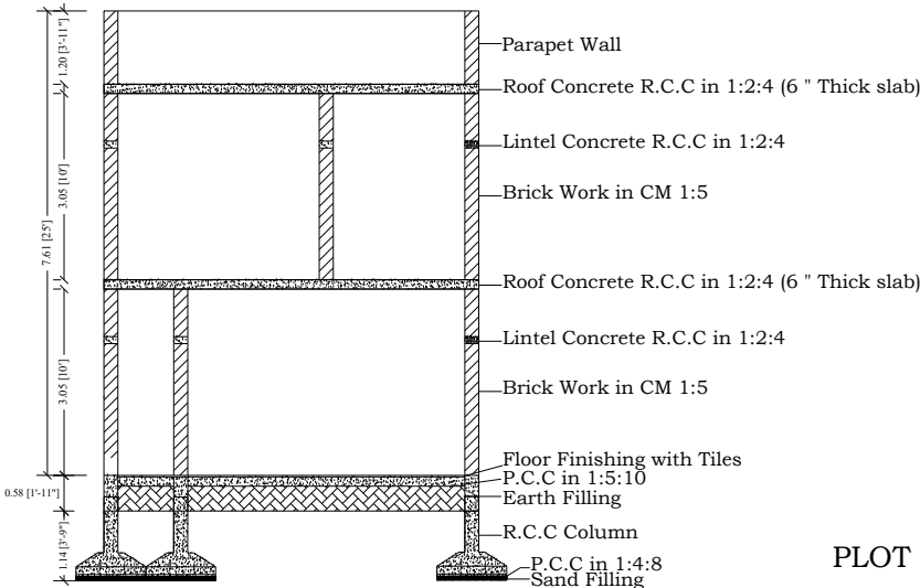
SECTION X-X
