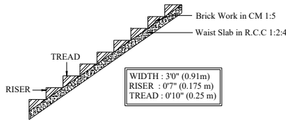
STAIRCASE DETAILS
