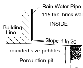
RAIN WATER HARVESTING:
