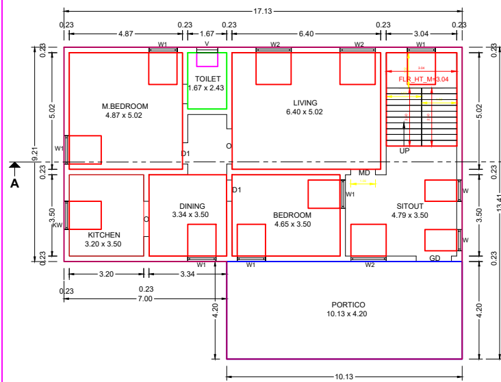
GROUND FLOOR PLAN (FLOOR-GROUND)
