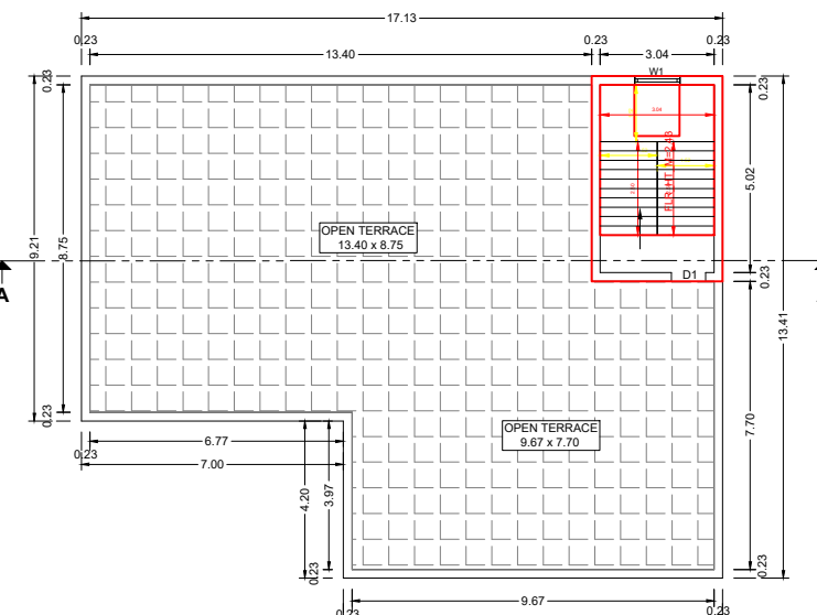
OPEN TERRACE PLAN (FLOOR-TERRACE)
