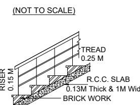
STAIRCASE DETAILS :-
