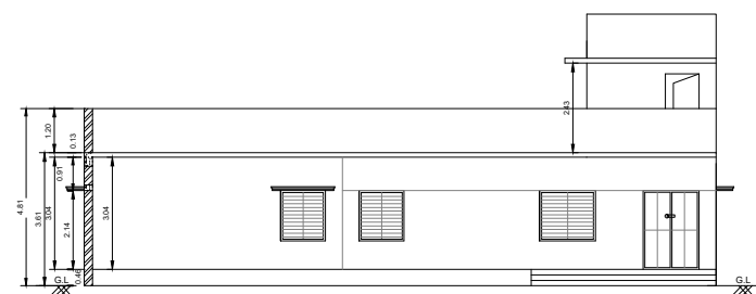
FRONT ELEVATION ON A-A
