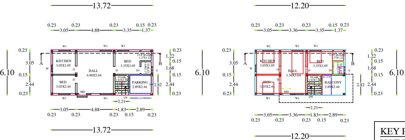
EXISTING APPROVED GROUND FLOOR PLAN NORTH FACING
