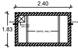
RAINWATER HARVESTING TRENCH
