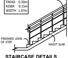
STAIRCASE DETAILS
