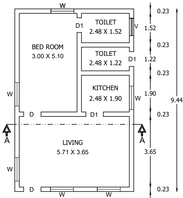
TYPICAL BLOCK 1,2- GROUND FLOOR
