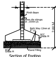
FOUNDATION DETAILS
