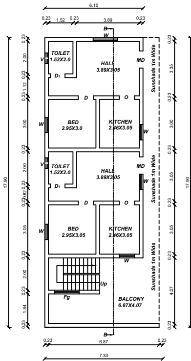
PROPOSED SECOND FLOOR PLAN
