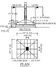
FOUNDATION DETAILS
