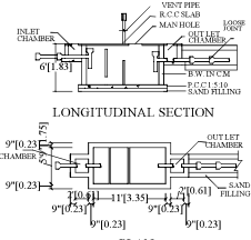
SEPTIC TANK
