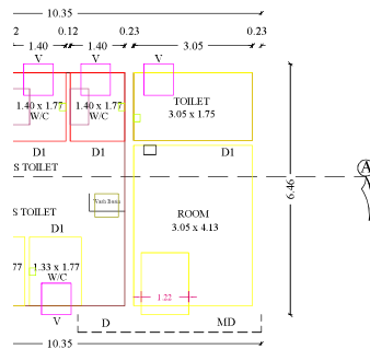
GROUND FLOOR PLAN (LOCK-02)
