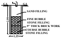
SECTION ON RAIN WATER COLLECTION TANK
