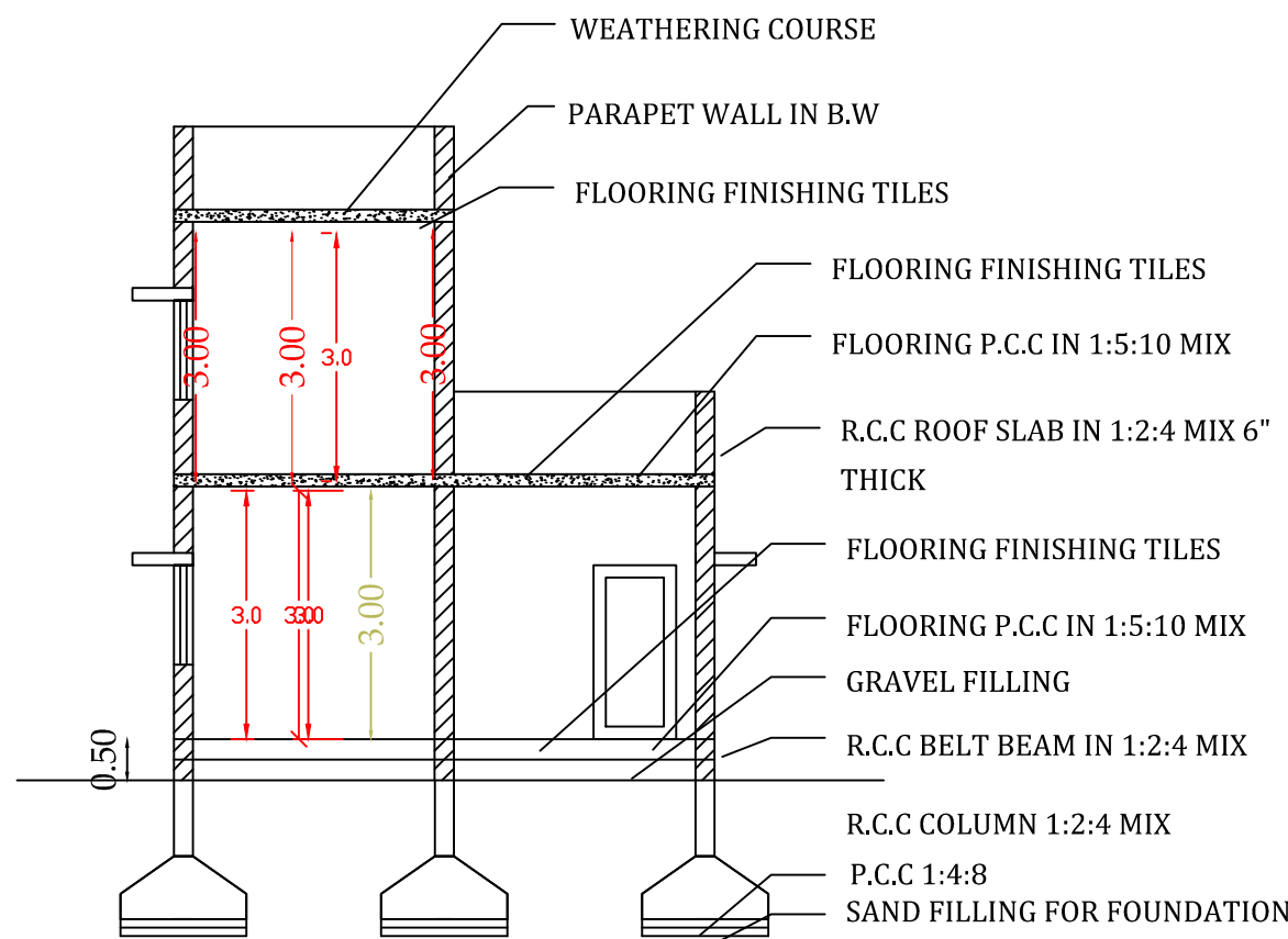
SECTION A TO B
