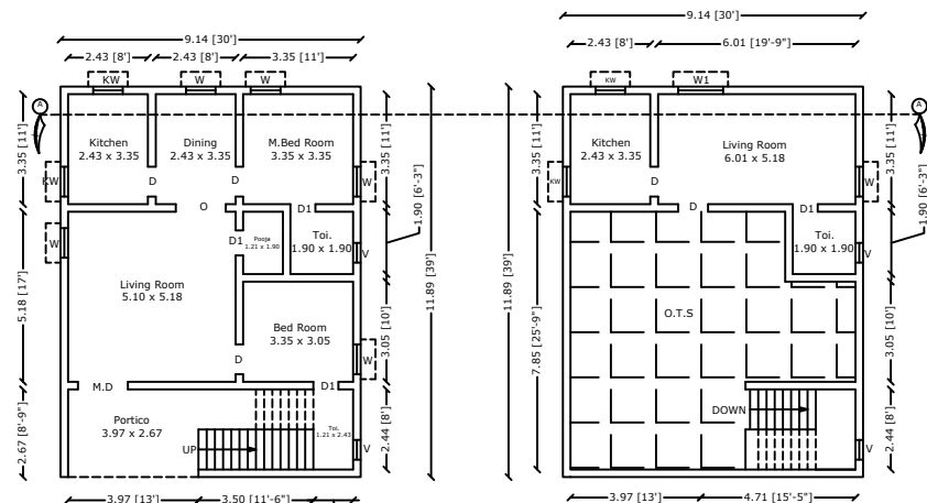
OPEN TERRACED FLOOR PLAN
