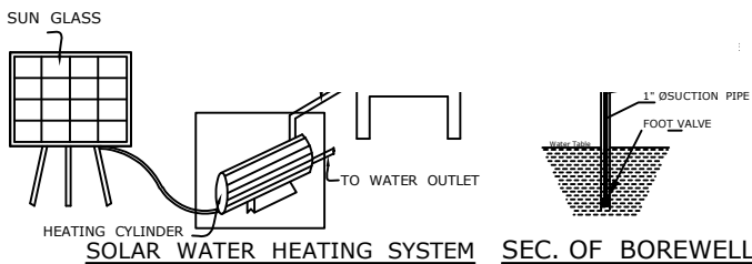
SOLAR WATER HEATING SYSTEM
