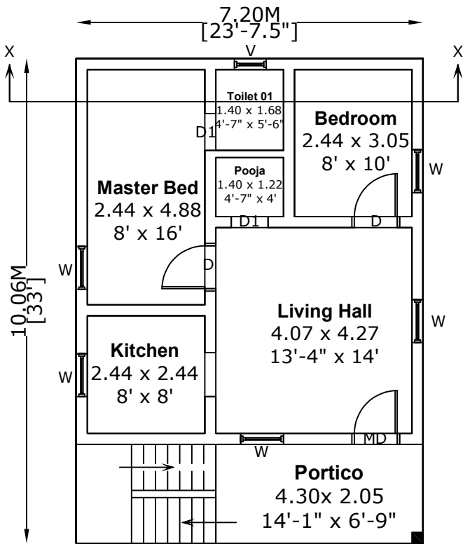
SITE CUM PRO.GROUND FLOOR
