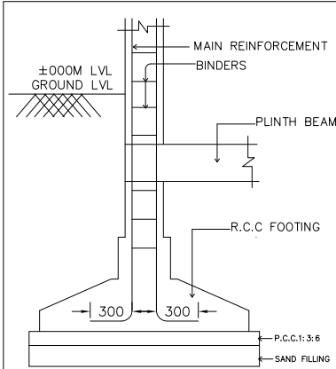
TYPICAL SECTION OF R.C.C COLUMN FOUNDATION
