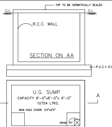
SUMP DETAIL
