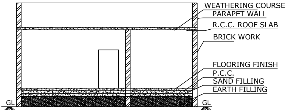
SECTION ON XX
