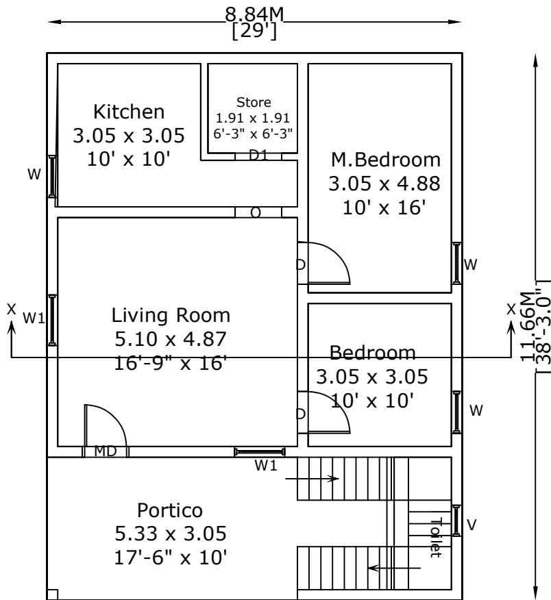
SITE CUM PRO.GROUND FLOOR
