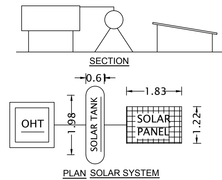
PLAN SOLAR SYSTEM
