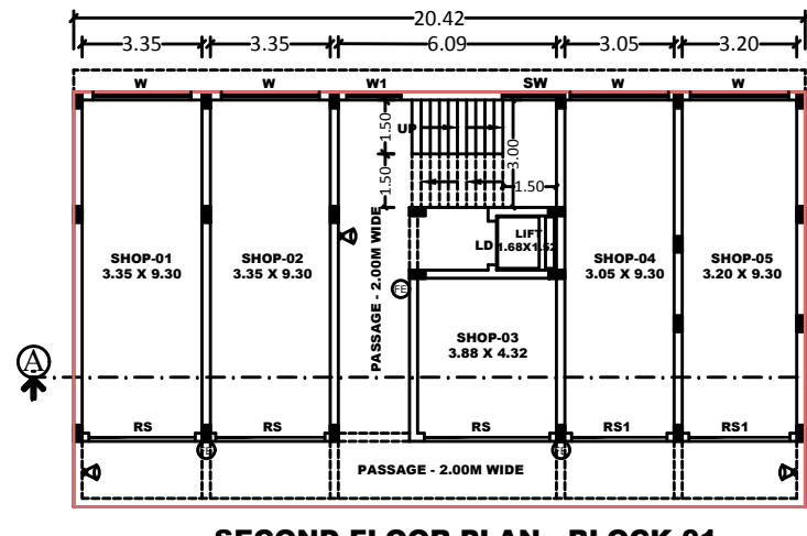
SECOND FLOOR PLAN - BLOCK 01 (Scale 1:100)
