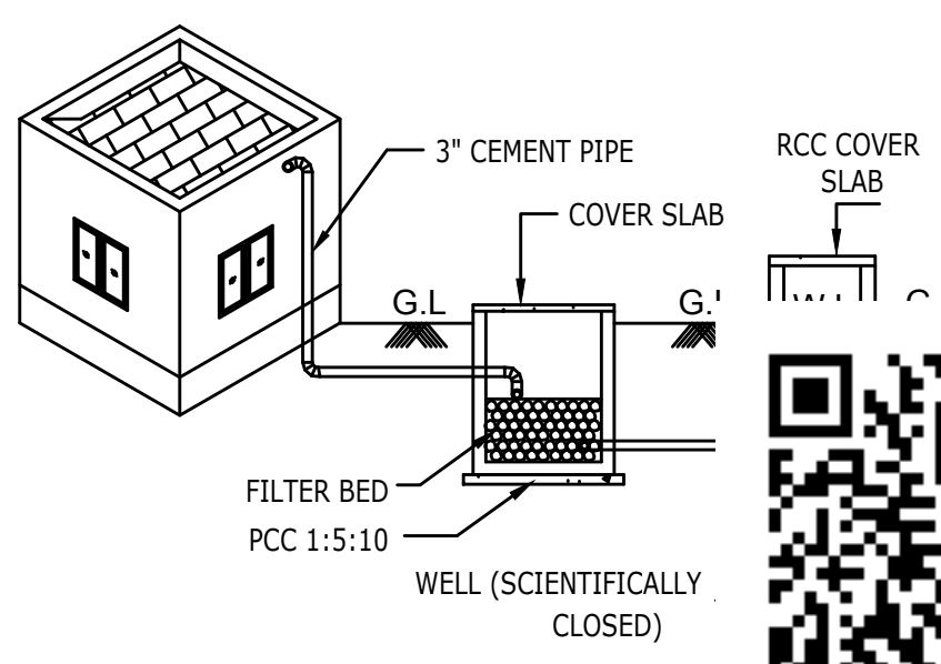
PROPOSED RAIN WATER HARVESTING CHAMBER
