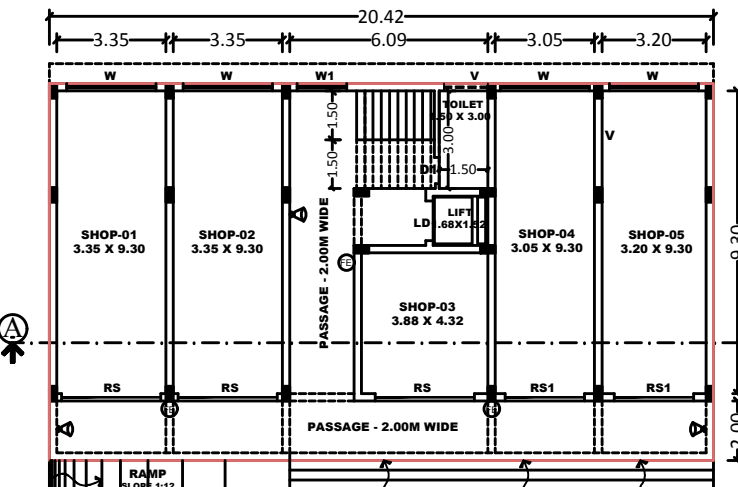
GROUND FLOOR PLAN - BLOCK 01 (Scale 1:100)
