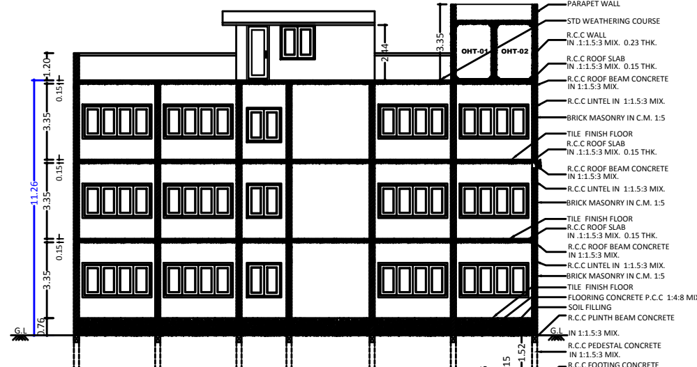
SECTION ON "AA" - BLOCK 01 (Scale 1:100)
