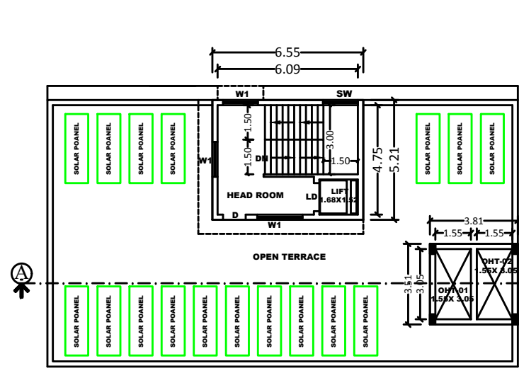
TERRACE FLOOR PLAN - BLOCK 01 (Scale 1:100)
