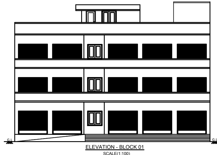
ELEVATION - BLOCK 01 (Scale 1:100)
