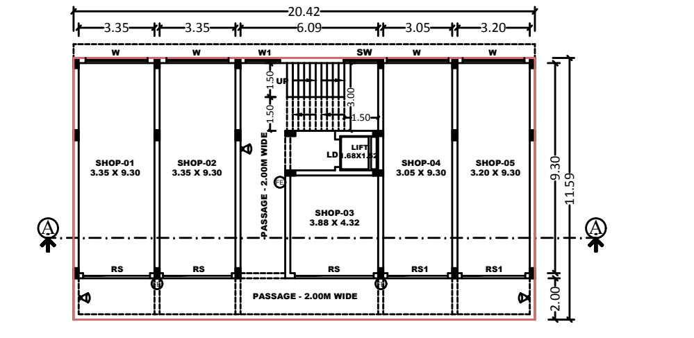
FIRST FLOOR PLAN - BLOCK 01 (Scale 1:100)
