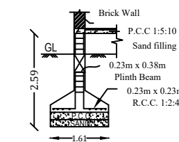
FOUNDATION DETAILS
