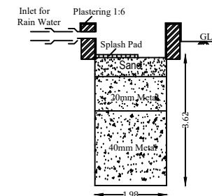
RAIN WATER PERCOLATION PIT
