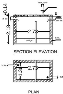
SEPTIC TANK
