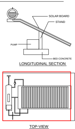
SOLAR WATER HEATER
