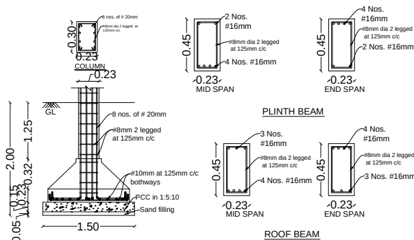
RCC COLUMN AND FOOTING
