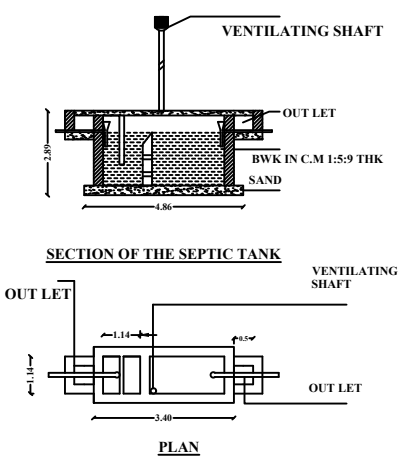
SEPTIC TANK
