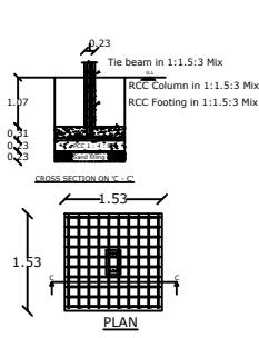
COLUMN FOUNDATION DETAILS:-
