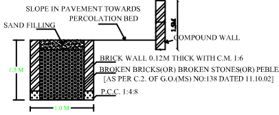
SECTION OF RAIN WATER PERCOLATION BED
