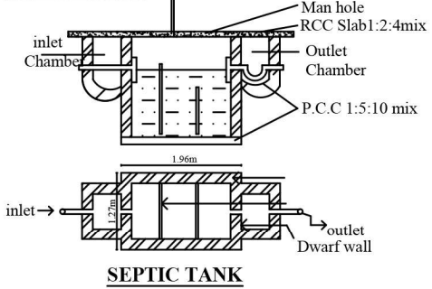
SEPTIC TANK
