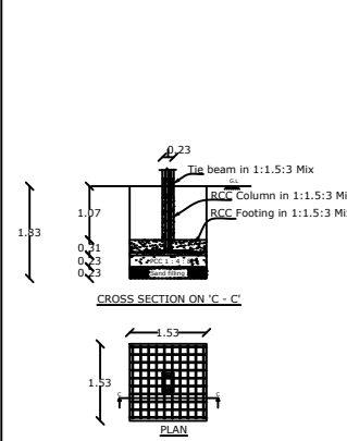
COLUMN FOUNDATION DETAILS:-
