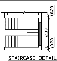
STAIRCASE DETAIL
