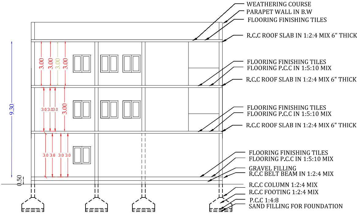
SECTION A TO B
