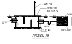
SEPTIC TANK & DISPERSION TRENCH DETAILS
