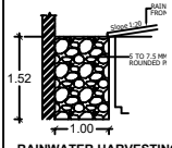
RAINWATER HARVESTING TRENCH
