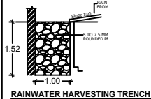
RAINWATER HARVESTING TRENCH
