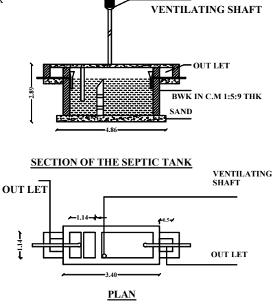
SEPTIC TANK
