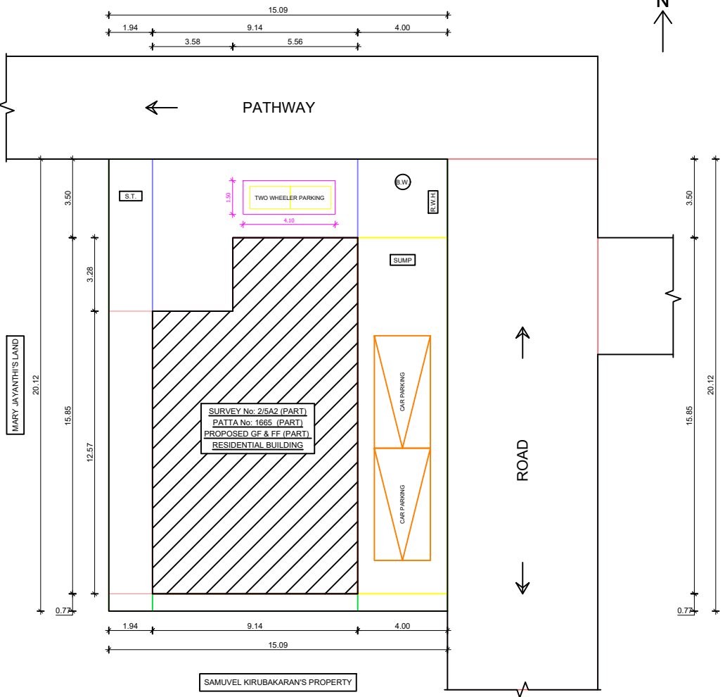
SITE PLAN
