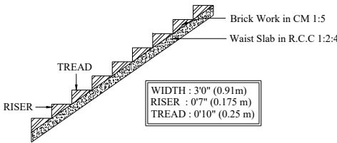
STAIRCASE DETAILS
