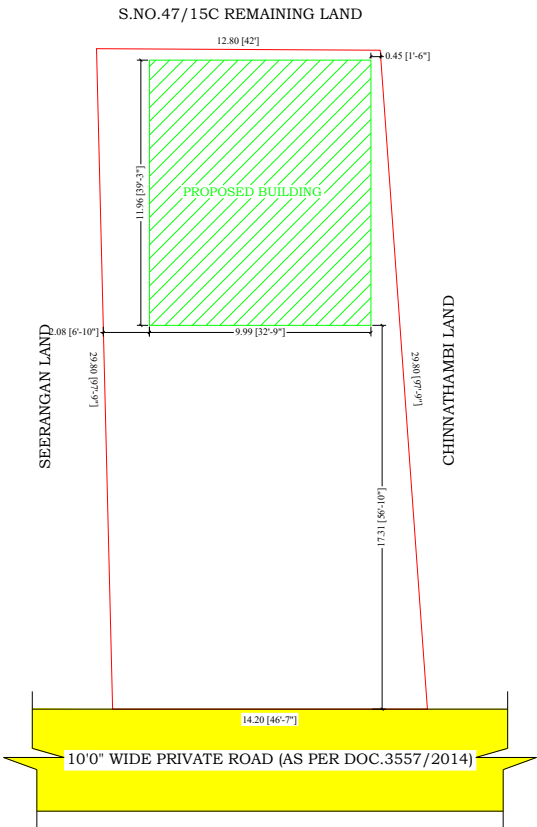
SITE PLAN (SCALE - 1:250)
