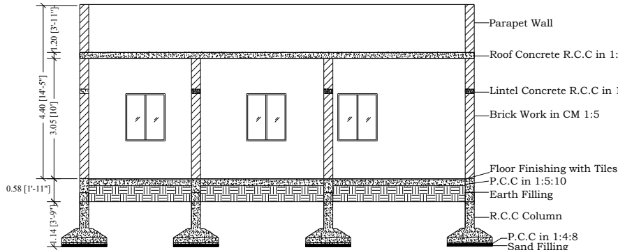
SECTION X-X
