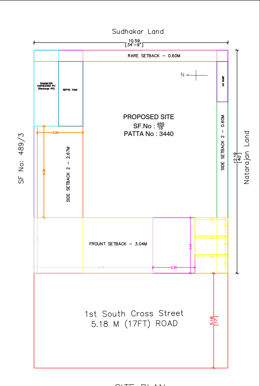
SITE PLAN
