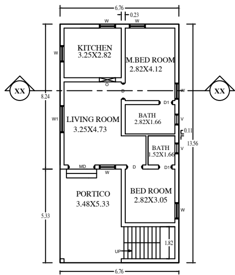
PROPOSED BUILDING OF GROUND FLOOR
