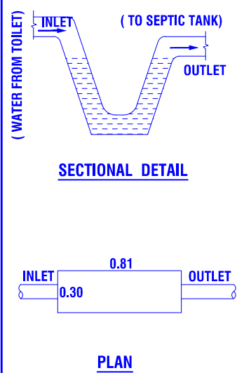
DETAILS OF "U" TRAP
