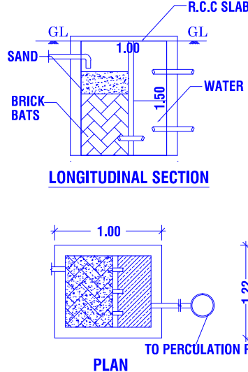
RAIN WATER HARVESTING TUB
