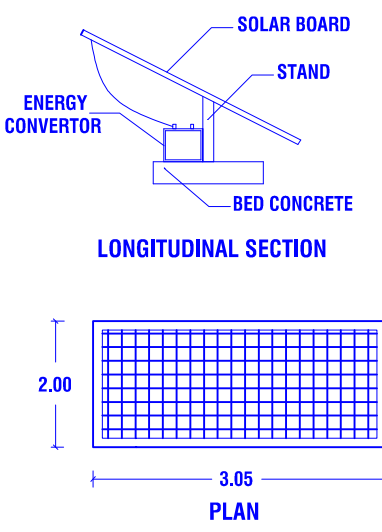
SOLAR PANEL
