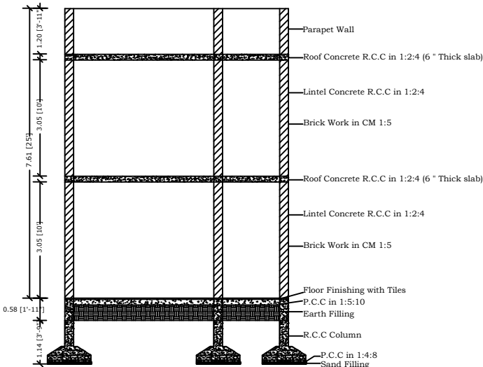
SECTION X-X
