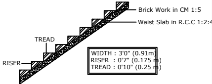
STAIRCASE DETAILS
