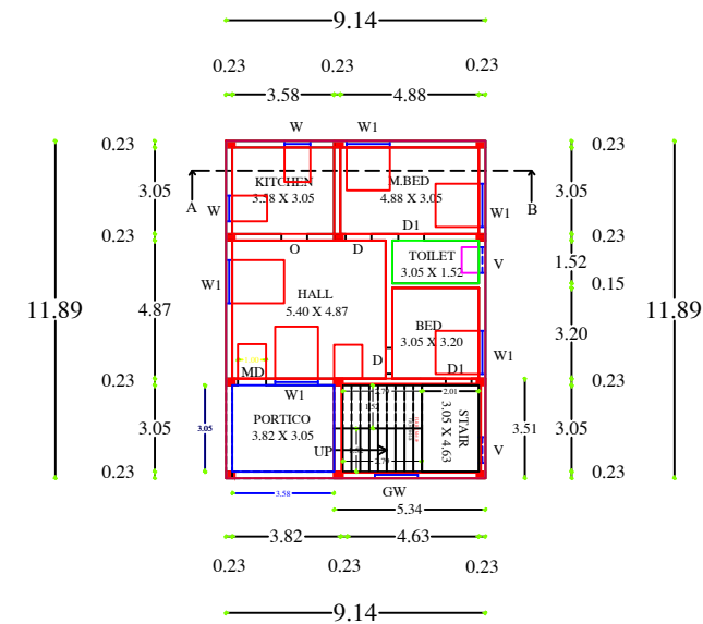
PRO.GROUND FLOOR PLAN NORTH FACING
