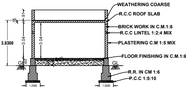
SECTION ON-"AB"
