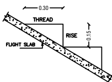
STAIRCASE DETAILS
