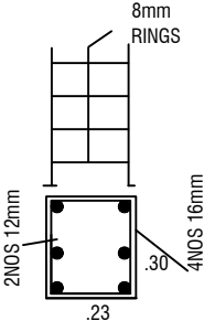
COLUMN DETAILS
