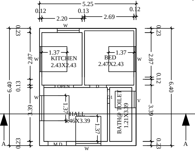
PLAN FOR GROUND FLOOR
